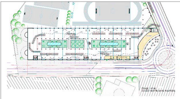
Ground floor plan bus station
